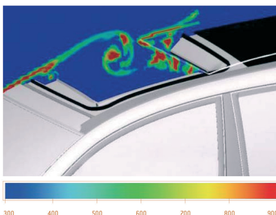
Simulation of the airflow above a sunroof (Mégane).
