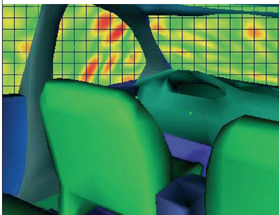
Velocity field on the windows of a Laguna subjected to airflow.
